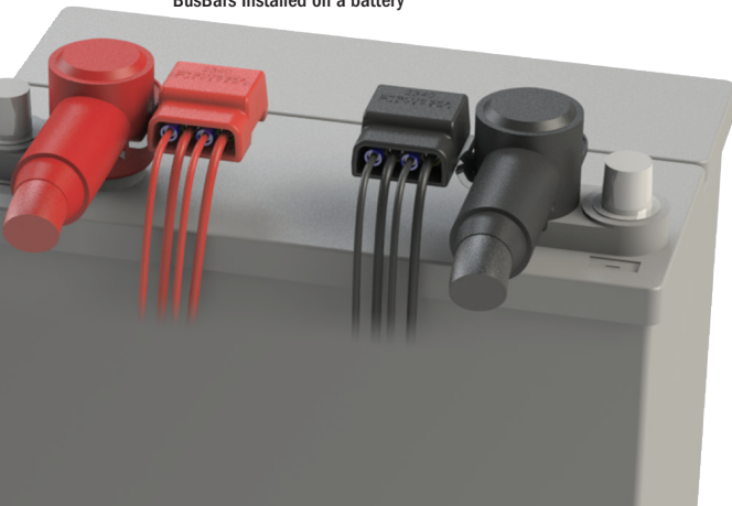
5026 12 circuit Positive and negative bus
